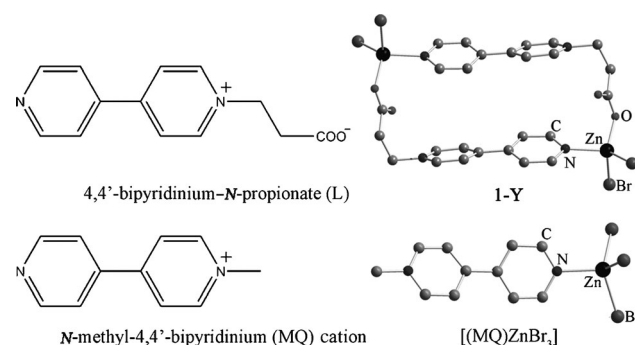
Figure 1. L and MQ ligands and molecular structures of 1-Y and [(MQ)ZnBr 3 ]. H atoms are omitted for clarity.
